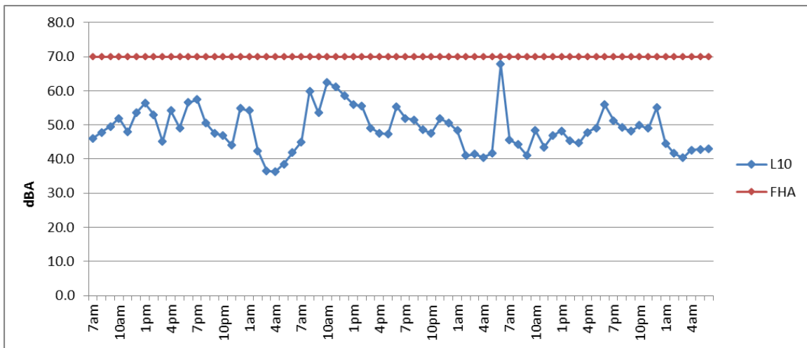
Figure 4.7: Comparison of L10 at Station 3 with FHA Standard
