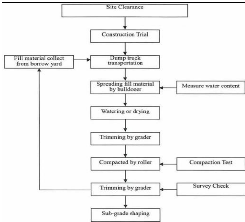
Figure 1.9: Construction Procedure for Roadbed Filling
