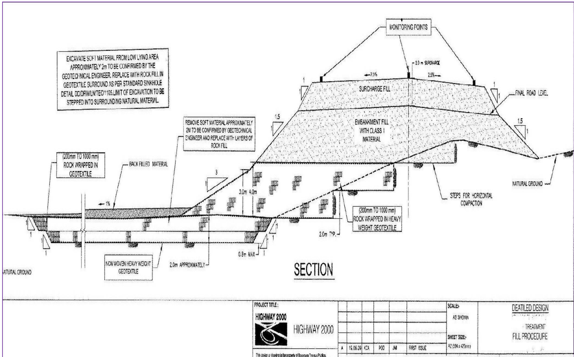
Figure 4.49: Treatment & Fill Procedure (Source: NROCC)
