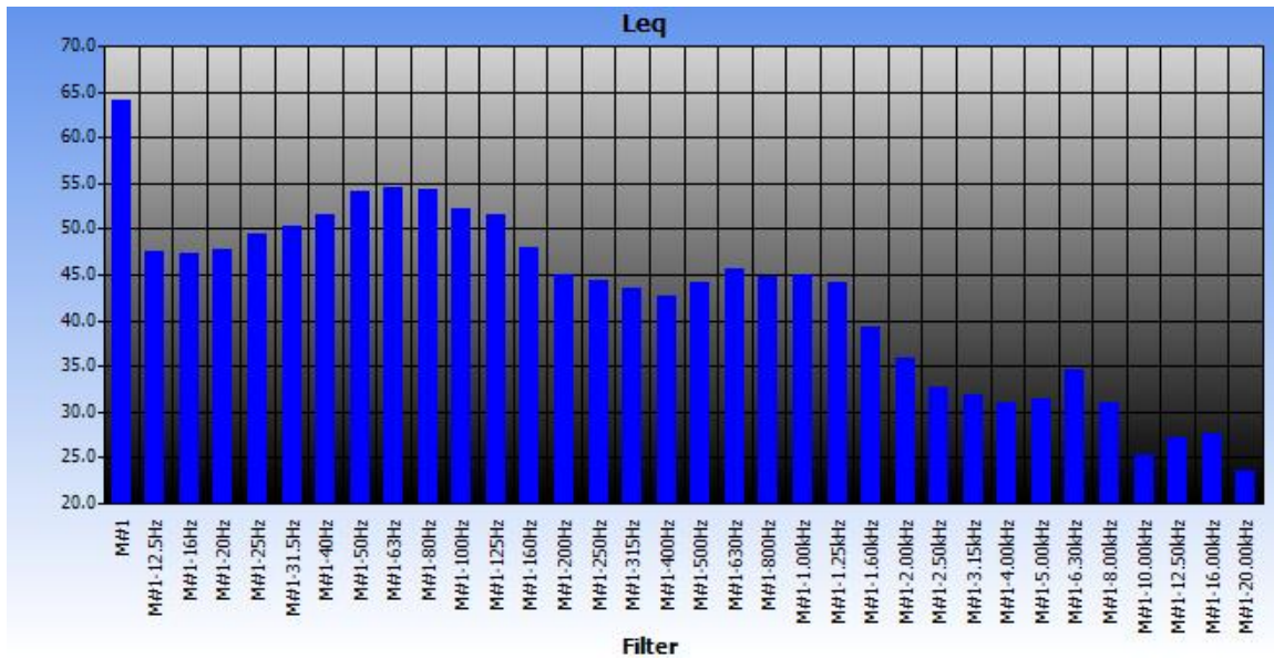
Figure 4.16: Octave band spectrum of noise at Station 2
