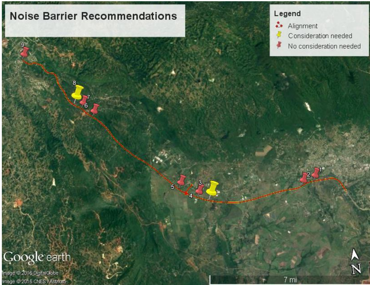
Figure 5.18: Noise Barrier Recommendation
