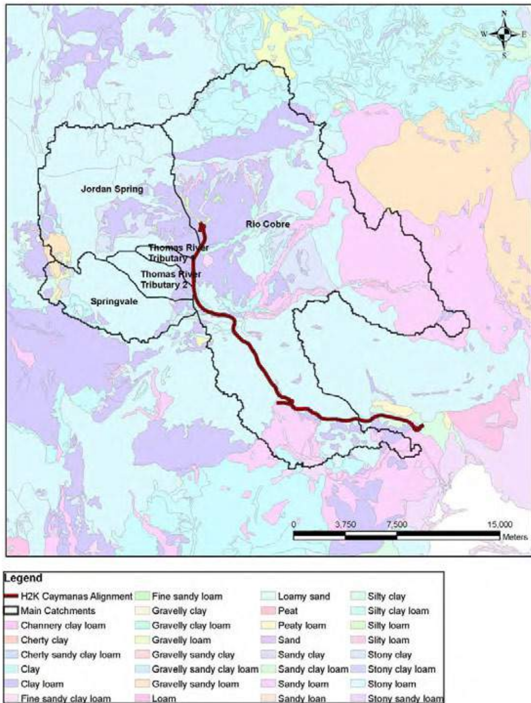
Figure 4-27 - Catchment areas superimposed on soils map of Jamaica
