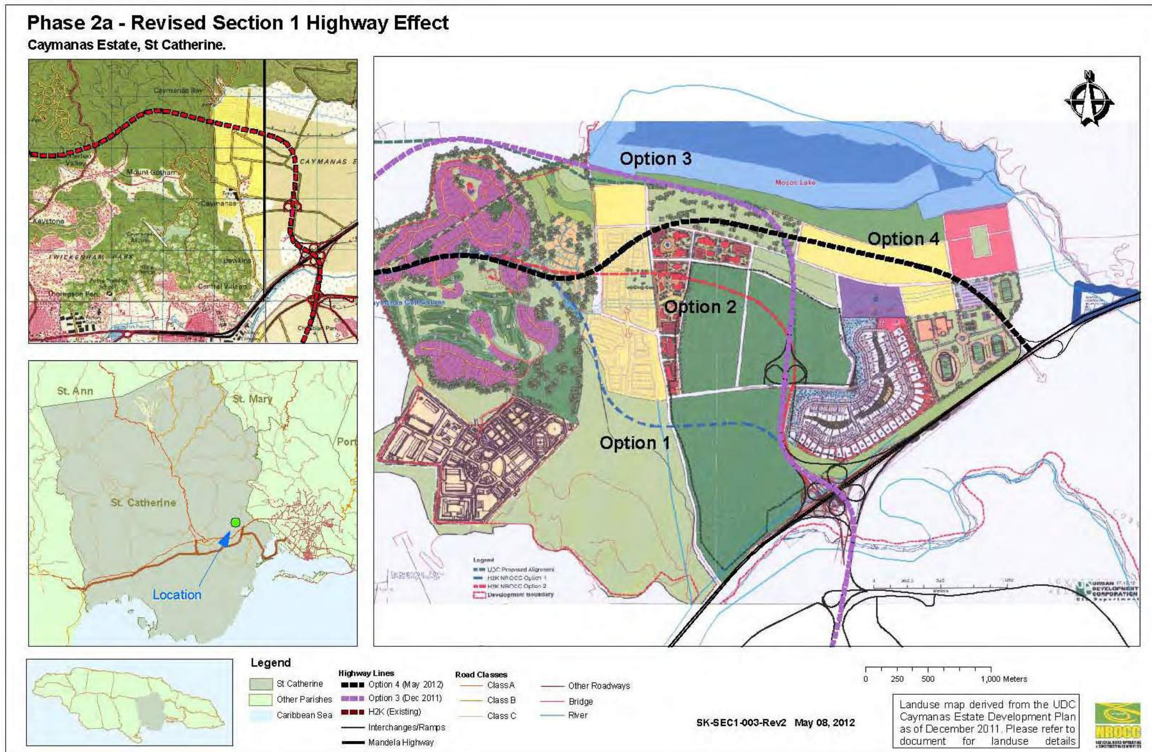
Figure 2-2 - The Caymanas to Linstead highway alignment through the Caymanas Estate (Option 4)
