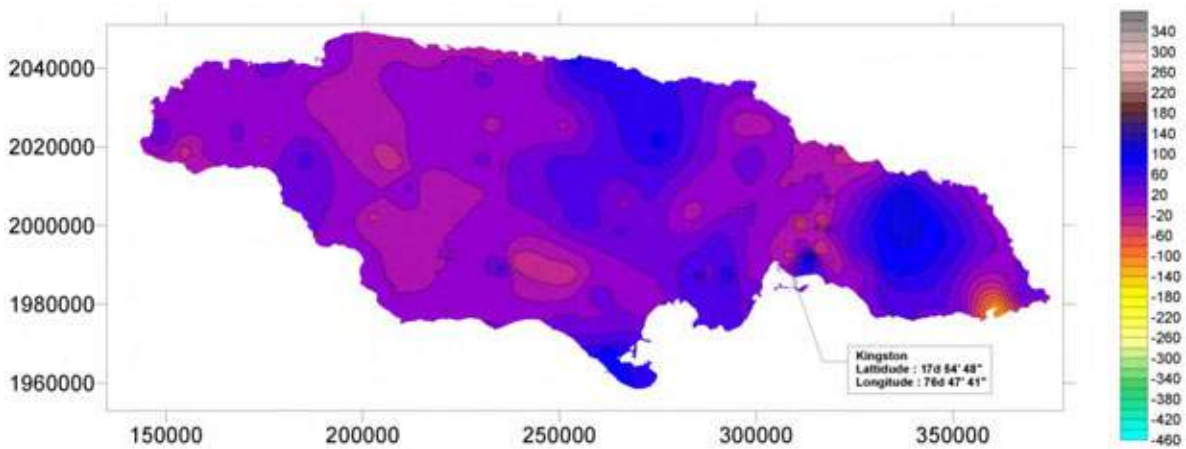
Figure 12-1 - Difference (mm) between the 1930-1988 and 1992 to 2008 24-hours Extreme rainfall intensities for the 2 Year Return Period Event
