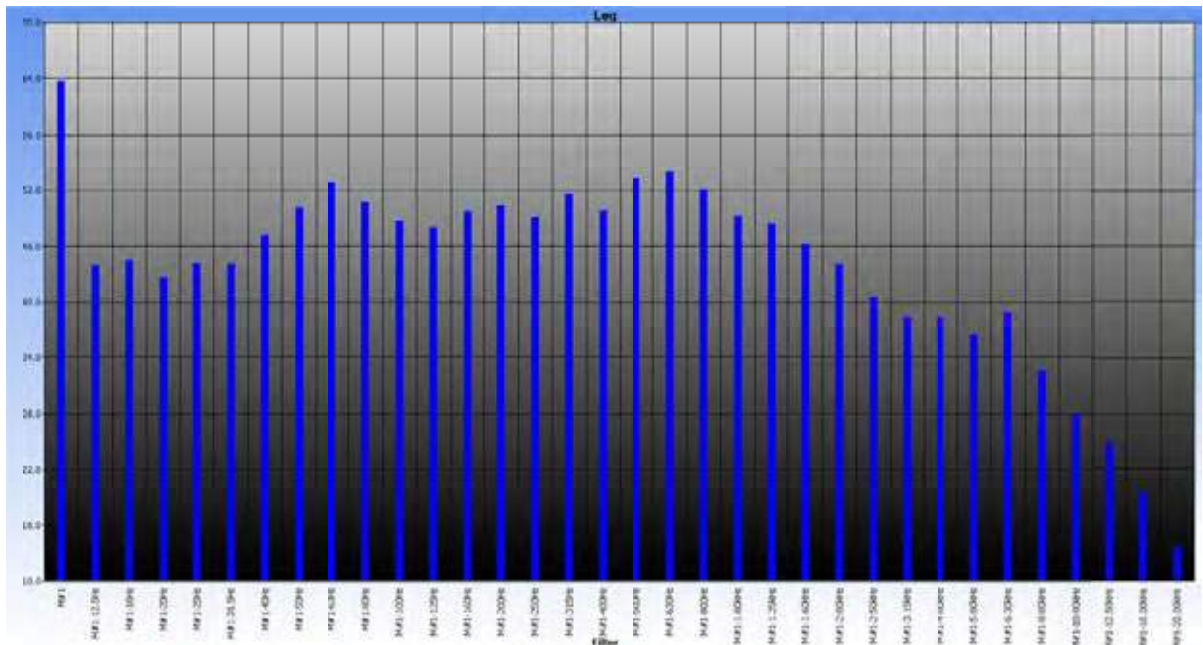
Figure 4-65 - Octave band spectrum of noise at Station 5
